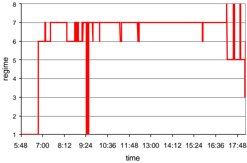
Figure 2 Classification of Traffic Conditions on SR-55 Northbound at Edinger Avenue, Postmile 9.41, Daytime Monday, March 2, 1998
